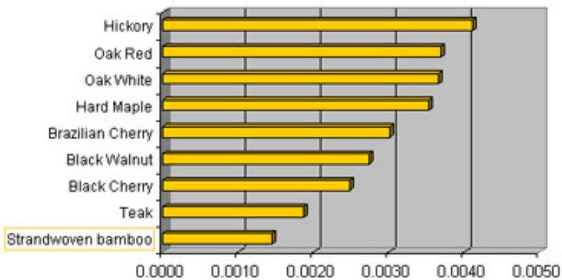
Dimensional Stability of Common Woods (smaller values indicate greater stability)
