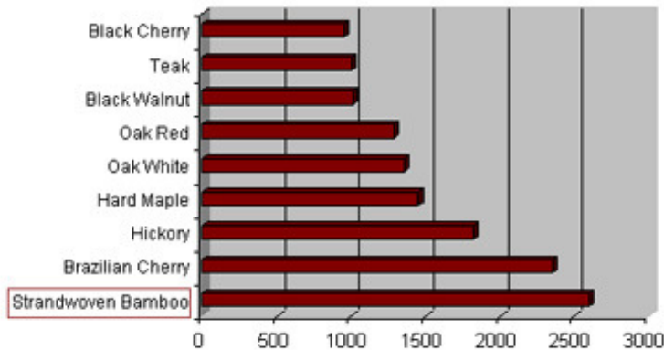
Hardness of Common Woods
